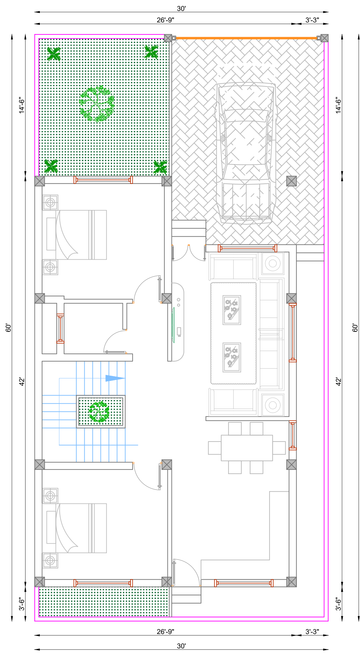
LANDSCAPE PLAN WITH GROUND FLOOR PLAN Plinth Area: 1123.50 Sq.Ft
