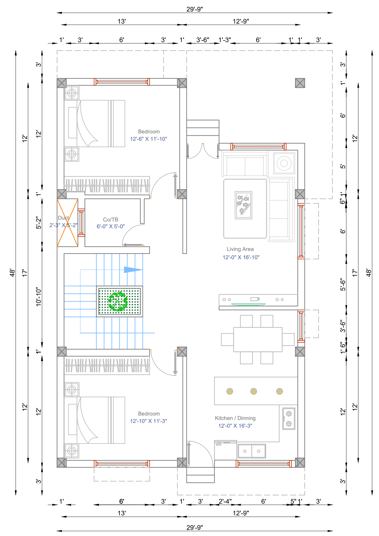
GROUND FLOOR PLAN Plinth Area: 1123.50 Sq.Ft
